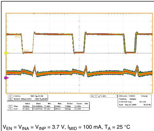
Figure 12. Line transient
