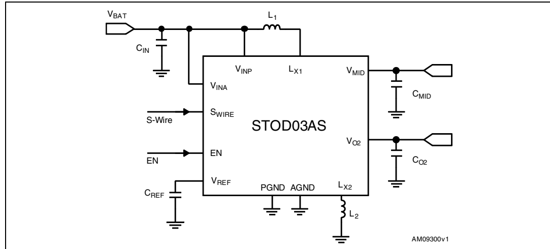
Figure 1. Application schematic
