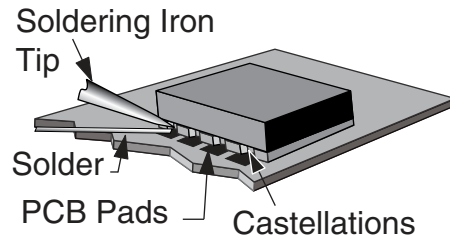
Figure 35: Soldering Technique
