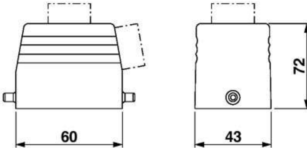
Dimensioned drawing
