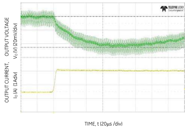
Figure 28. Transient Response to Dynamic Load Change from 50% to 100% at 12V in , C out =2x47uF+1x330uF, CTune=6800pF, RTune=300
