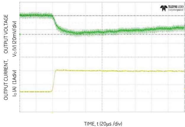
Figure 16. Transient Response to Dynamic Load Change from 50% to 100% at 12Vin, C_{out}=4 \times 47 \mu F + 1 \times 330 \mu F , C_{Tune}=15nF , R_{Tune}=300
