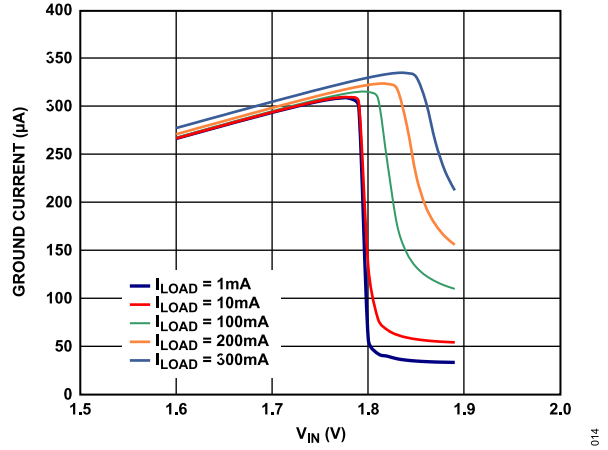
Figure 12. Ground Current vs. Input Voltage (in Dropout)
