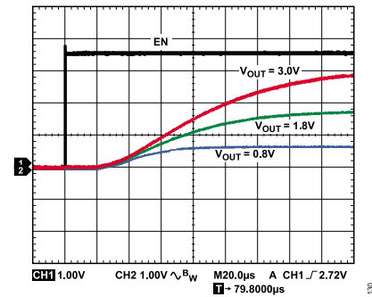
Figure 29. Typical Start-Up Time
