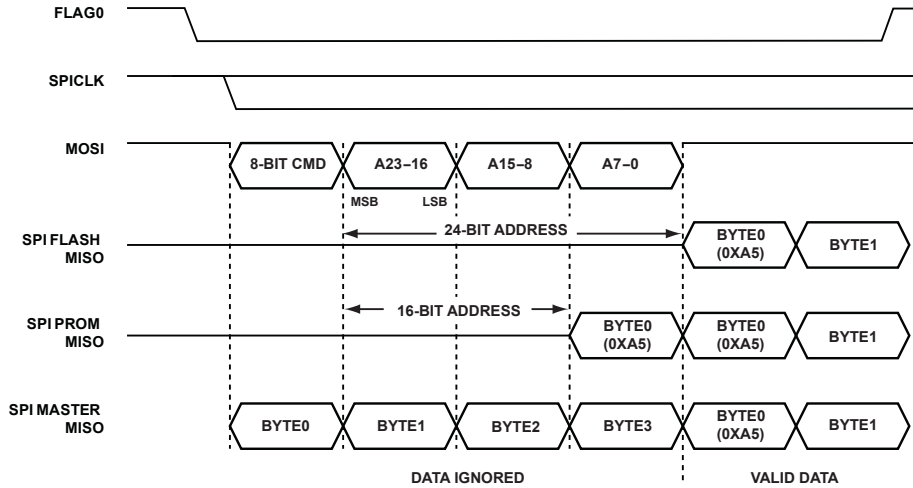
Figure 13. SPI Master Mode Booting Using Various Serial Devices
