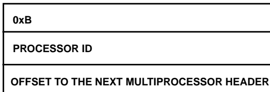
Figure 15. Multiprocessor Header
