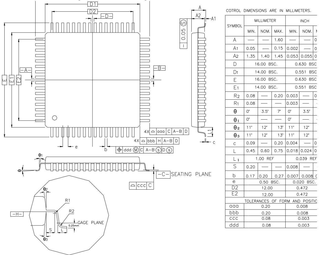
Figure 13-1. 100-lead LQFP Package Mechanical Drawing
