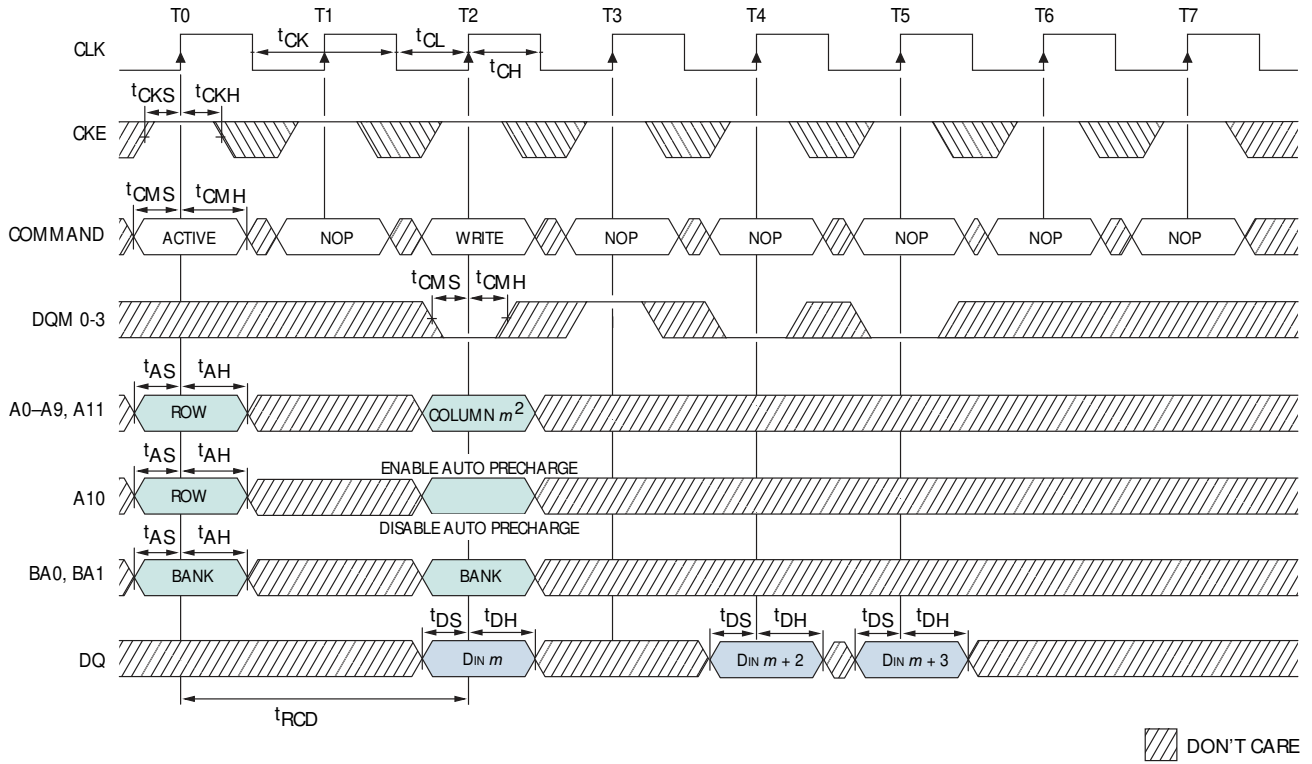
Figure 52: Write – DQM Operation 1
