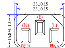
ME-302 (IEC 60320, C13) (Dimensions of Connector Face)
