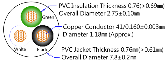
SJT 18AWGx3c 截面圖 (Wire Cross-Section)
