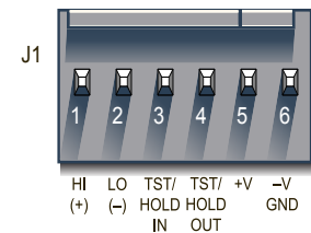
Figure 2. J1 Connector Pinout
