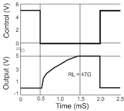
Fig. 12: Turn-on/Turn-off Characteristics
