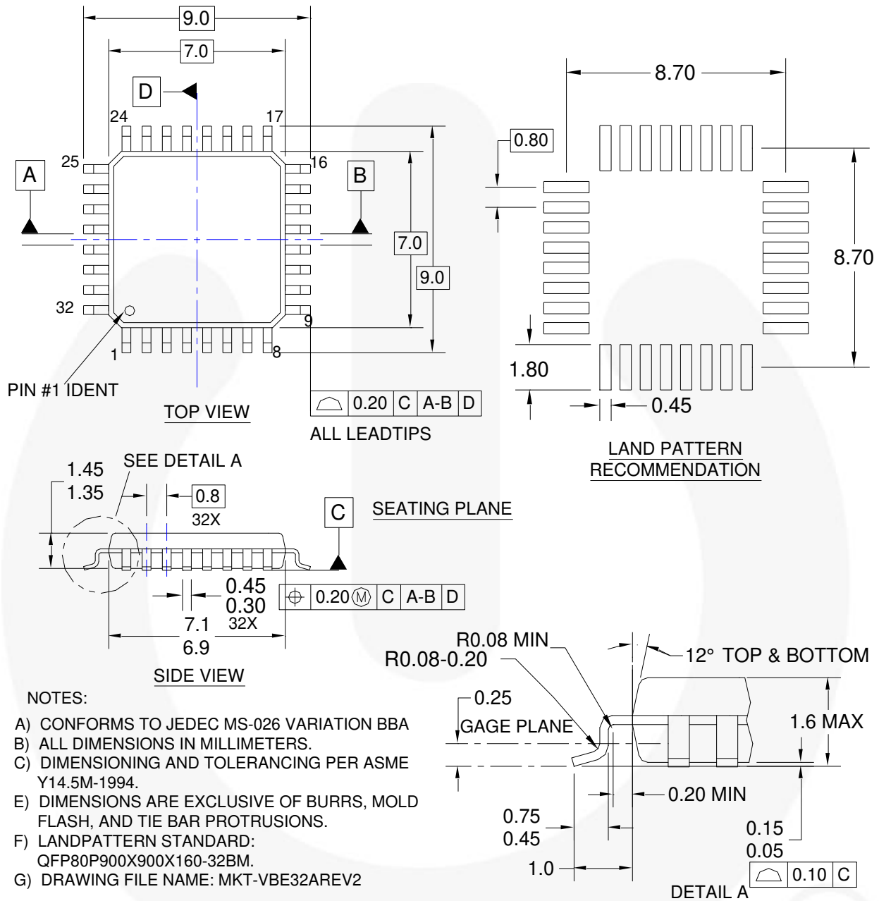
Figure 25. 32-Lead, Low-Profile, Quad Flat Pack Package (LQFP)
