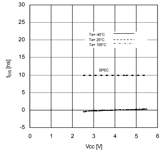
Figure 21. SI Setup Time vs Supply Voltage
