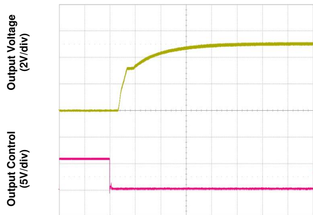
Figure 6. Start-Up from Enable Control
