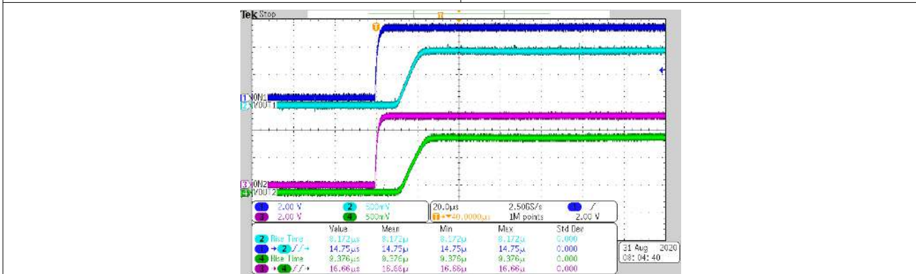
V_{IN} = 1.05\text{ V} V_{BIAS} = 5\text{ V} C_T = 0\text{ pF} Figure 7-42. Turnon Response Time
