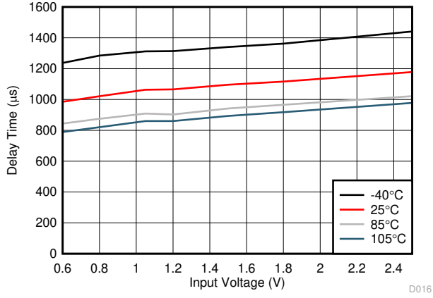
Figure 7-16. Delay Time vs Input Voltage
