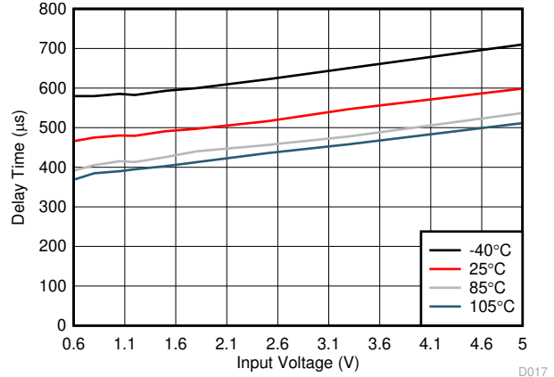
Figure 7-17. Delay Time vs Input Voltage
