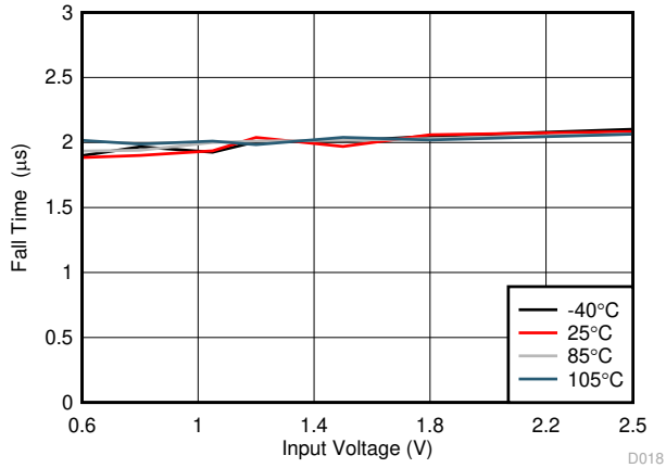
Figure 7-18. Fall Time vs Input Voltage
