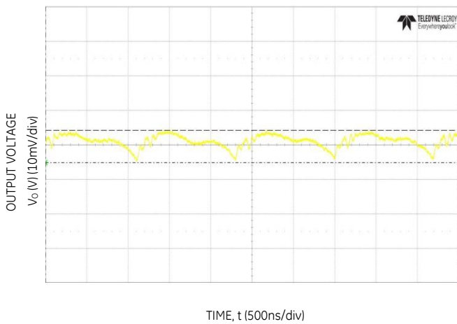
Figure 9. Typical output ripple (Co=2x47µF ceramic, Vin = 12V, Io = Io,max, ).
