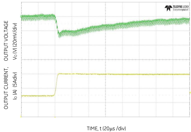
Figure 34. Transient Response to Dynamic Load Change from 50% to 100% at 12Vin, C_{out}=2\times 47\mu\text{F}+1\times 330\mu\text{F} , C_{Tune}=2700\text{pF} , R_{Tune}=300\Omega
