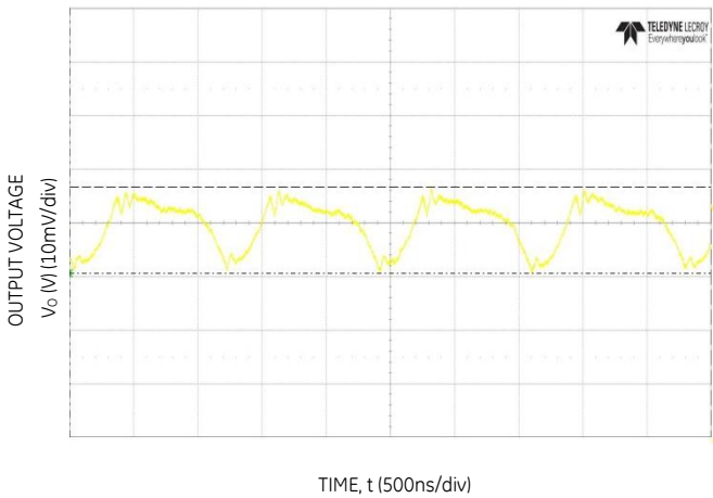
Figure 27. Typical output ripple (C o =2x47μF ceramic, V IN = 12V, I o = I o,max ).
