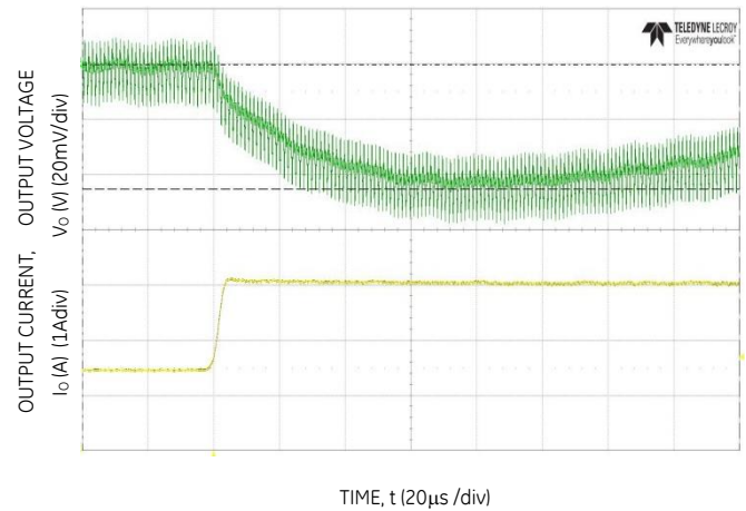
Figure 28 Transient Response to Dynamic Load Change from 50% to 100% at 12Vin, Cout=2x47uF+1x330uF, CTune=6800pF, RTune=300
