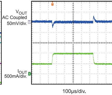
Transient Response
