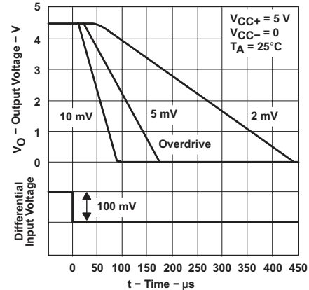
Figure 26. High-to-Low-Level Output Response for Various Input Overdrives
