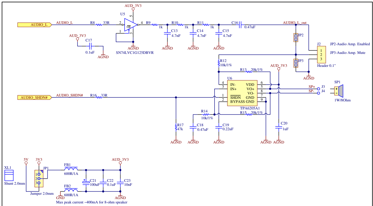
Figure 4-4 – VM800C Audio
