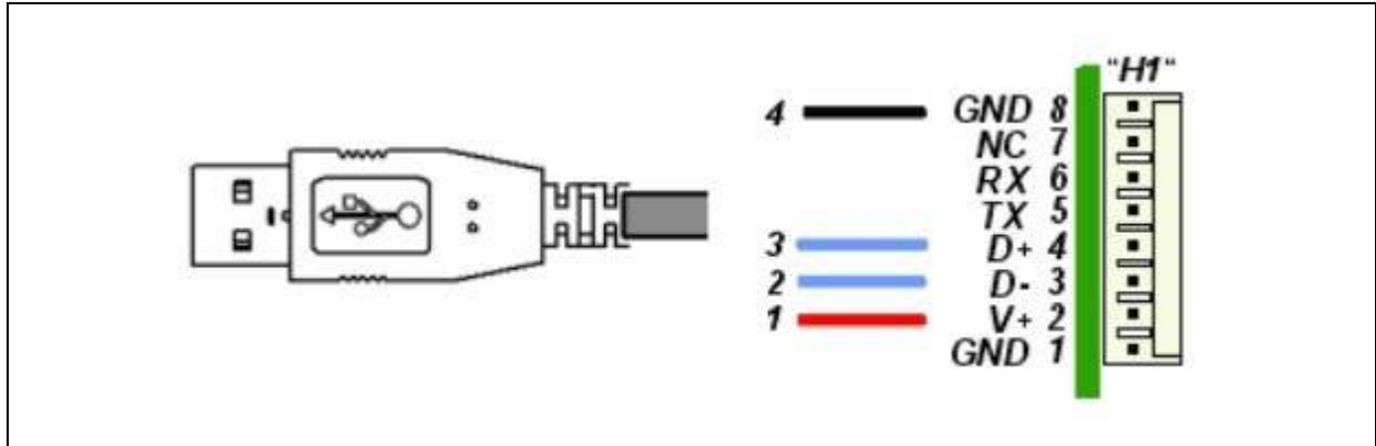
FIGURE 2-4: USB
