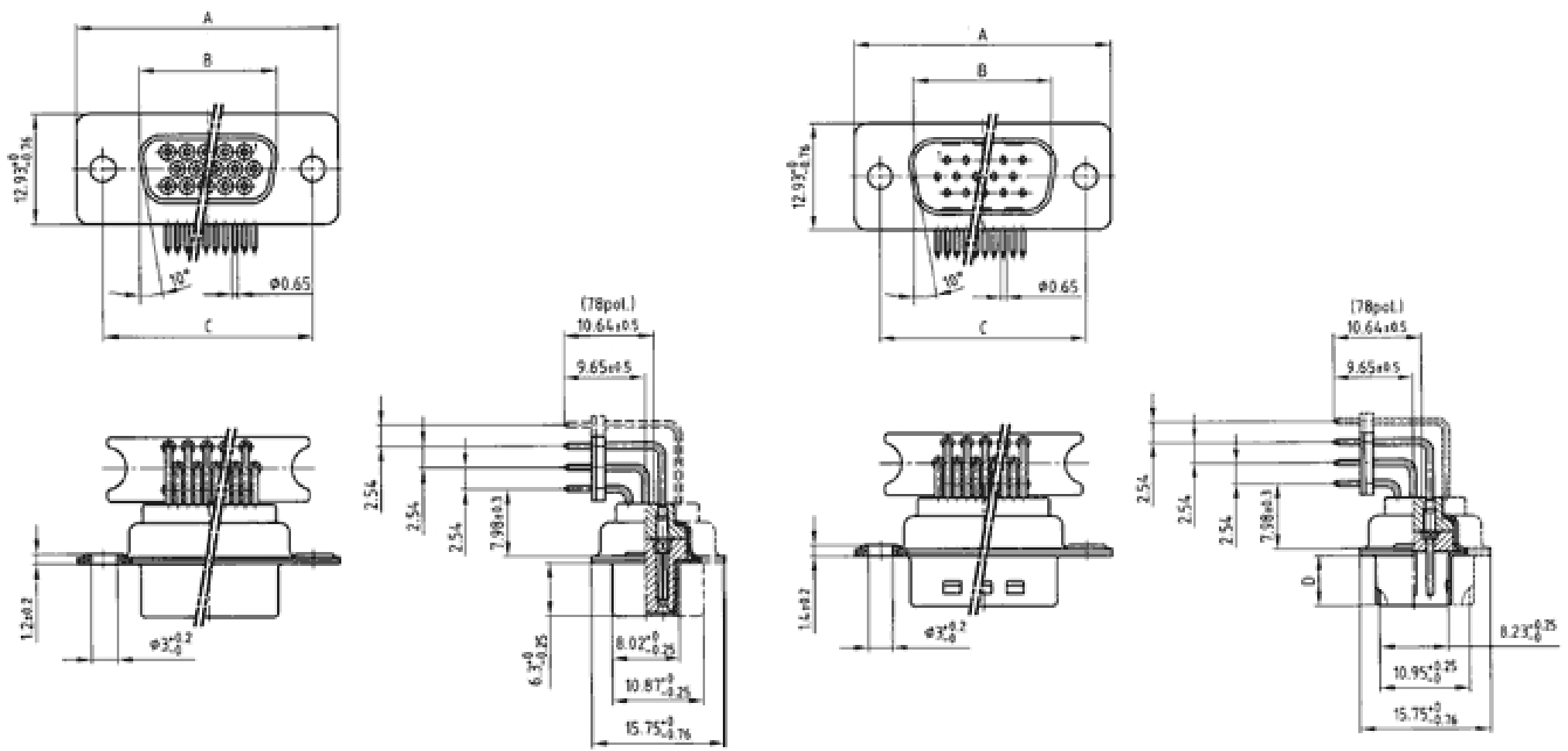
Socket connector:
