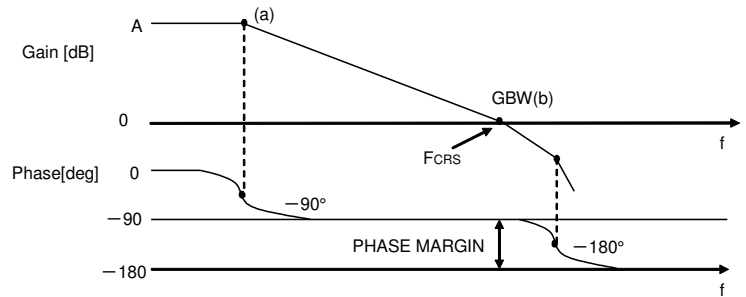
Figure 52. Bode Plot
