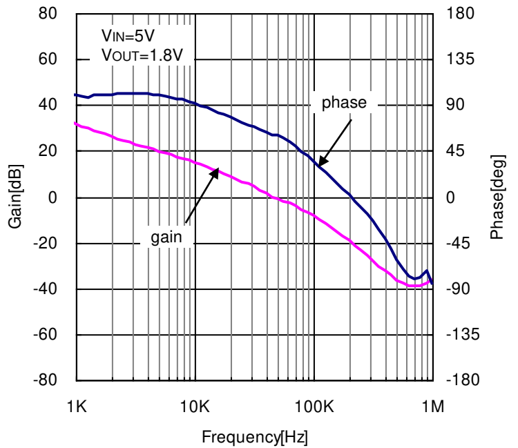
Figure 25. Closed Loop Response (VIN=5V, VOUT=1.8V, L=2.2μH, COUT=Ceramic 44μF)
