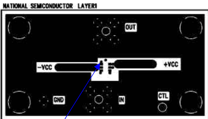
Sot23-6 Evaluation Board – Layer 1
