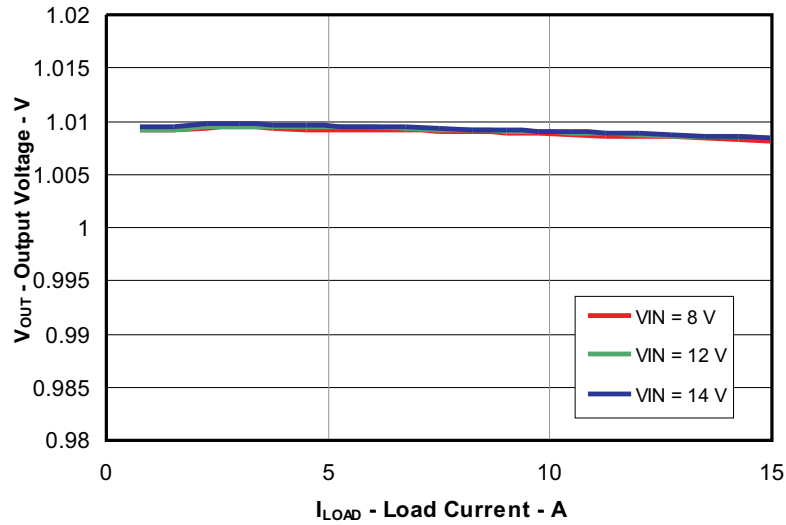
Figure 9-2. Load Regulation
