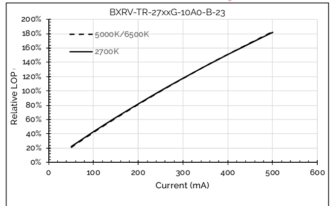
Figure 4: Relative Flux vs. Drive Current, T_c=25^\circ\text{C}
