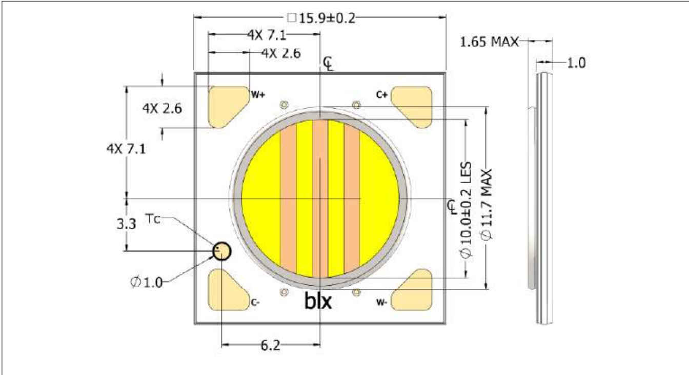
Figure 30: Drawing for Vesta Series Tunable White Gen2 9mm Array
