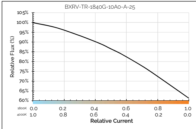
Figure 23: Relative Flux vs. Relative Current
