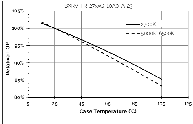
Figure 7: Relative Flux vs. Case Temperature
