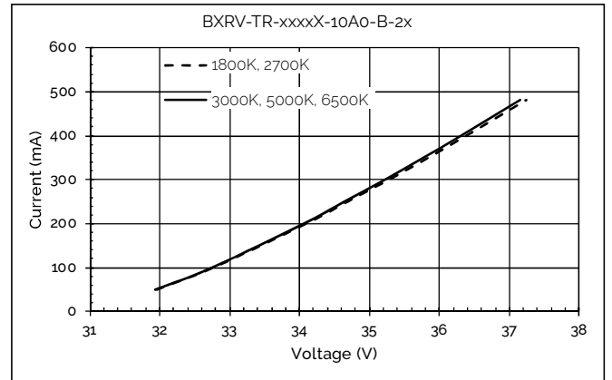
Figure 2: Forward Voltage vs. Forward Current, T_c=25^\circ\text{C}
