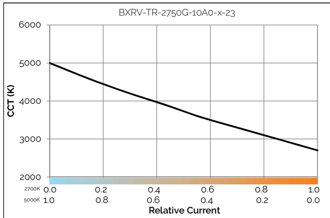
Figure 13: CCT vs. Relative Current, Tc=85C
