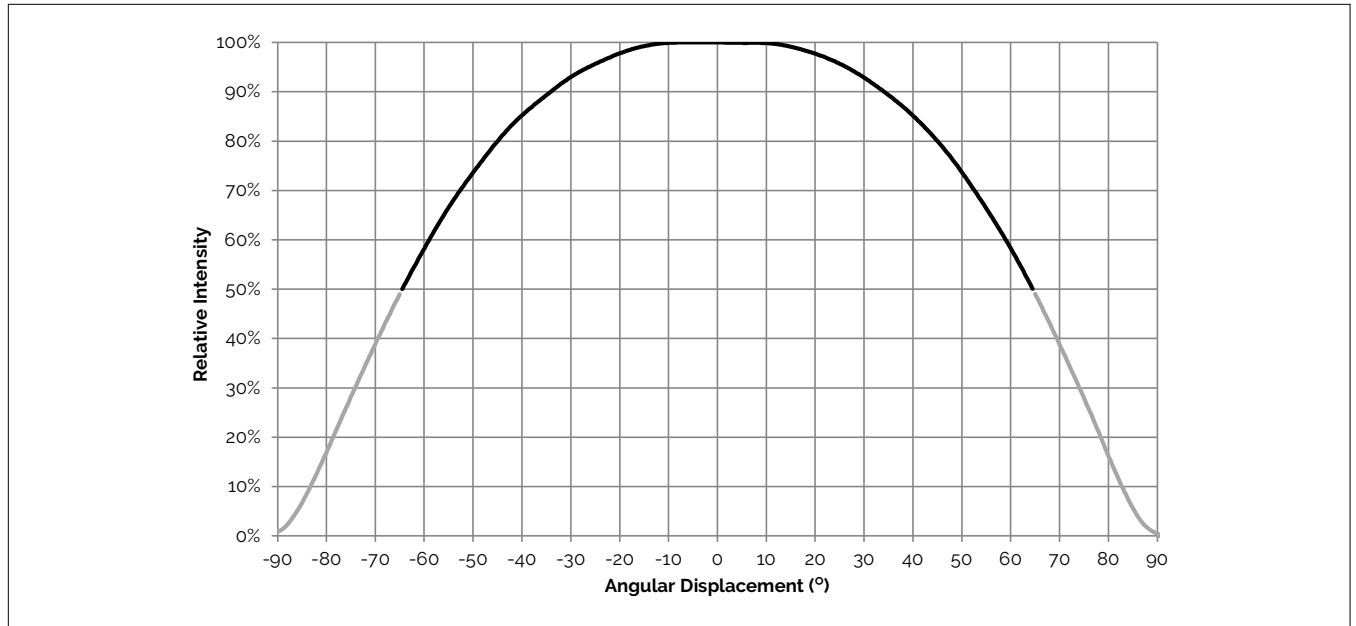
Figure 24: Typical Spatial Radiation Pattern
