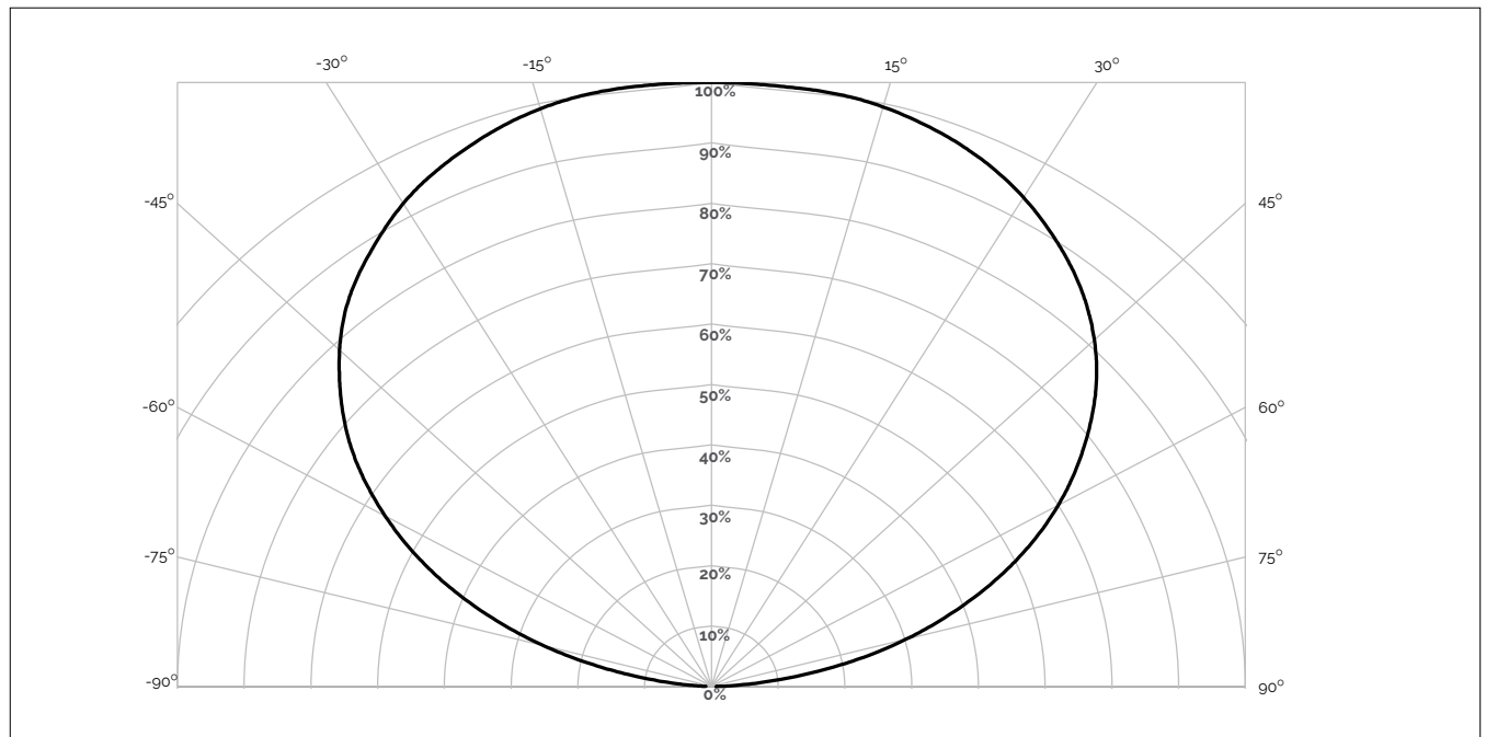
Figure 25: Typical Polar Radiation Pattern
