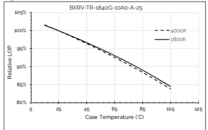
Figure 10: Relative Flux vs. Case Temperature
