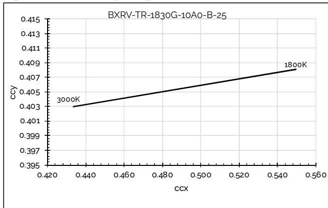
Figure 19: CCT Tuning Range, Tc=85C
