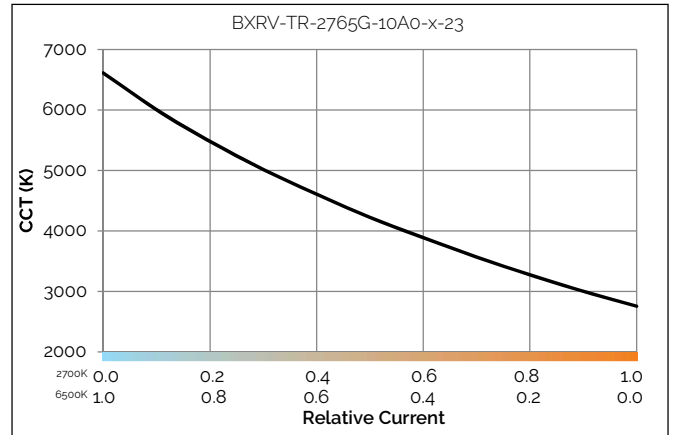
Figure 14: CCT vs. Relative Current, Tc=85C
