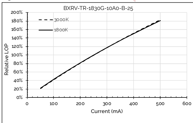
Figure 5: Relative Flux vs. Drive Current, T_c=25^\circ\text{C}
