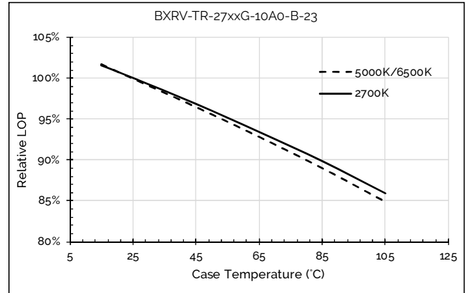
Figure 8: Relative Flux vs. Case Temperature
