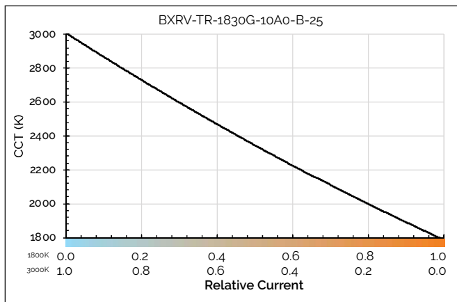
Figure 15: CCT vs. Relative Current, Tc=85C
