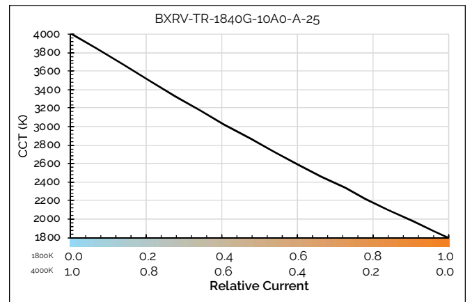
Figure 16: CCT vs. Relative Current, Tc=85C
