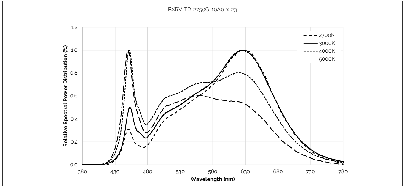
Figure 26: Typical Color Spectrum
