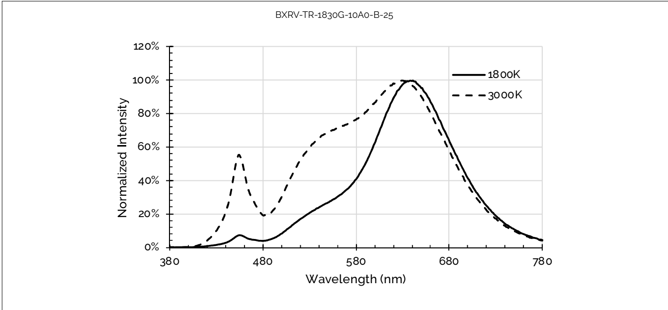
Figure 28: Typical Color Spectrum
