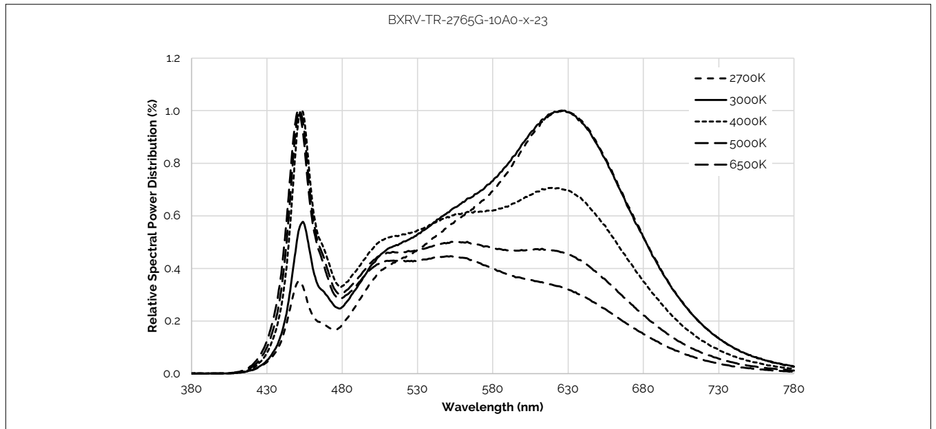
Figure 27: Typical Color Spectrum
