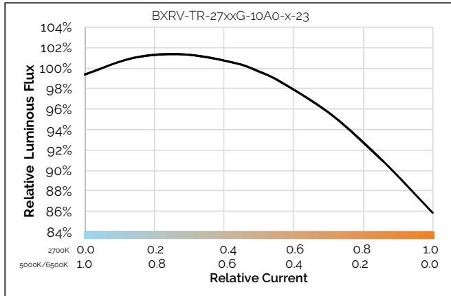
Figure 21: Relative Flux vs. Relative Current
