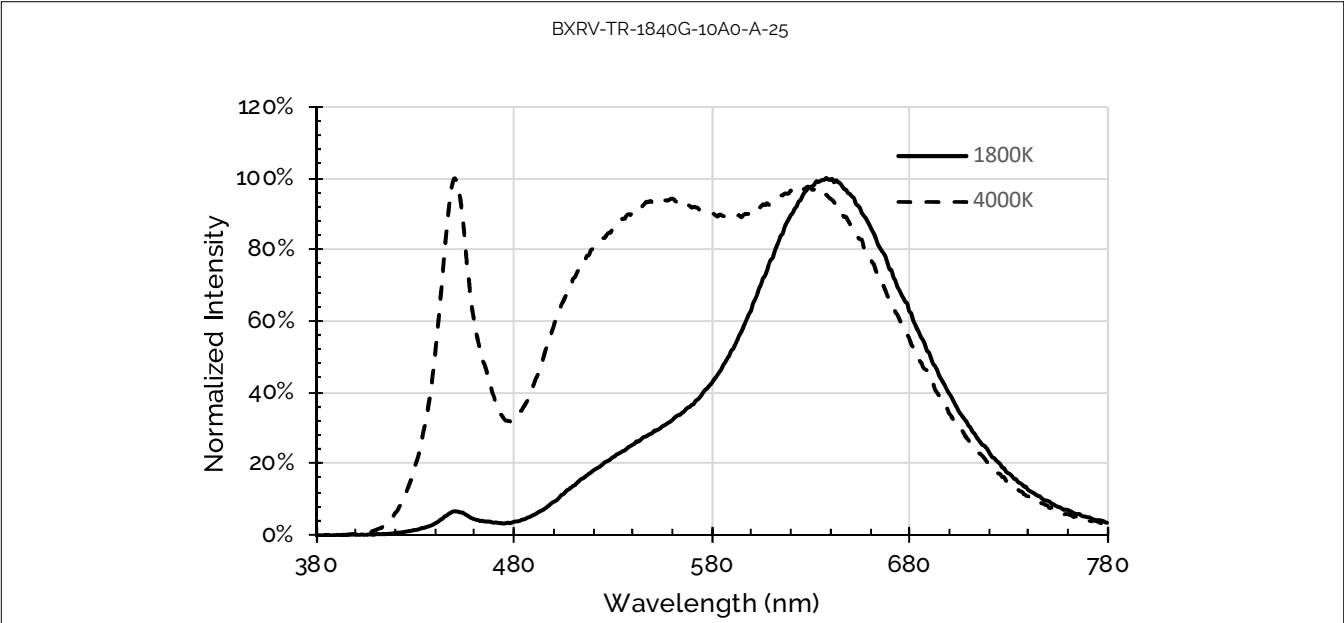
Figure 29: Typical Color Spectrum
