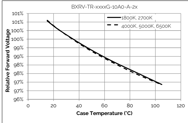
Figure 11: Relative Voltage vs. Case Temperature
