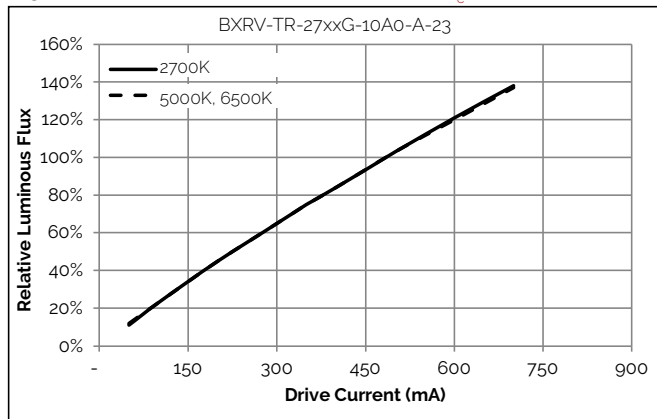
Figure 3: Relative Flux vs. Drive Current, T_c=25^\circ\text{C}
