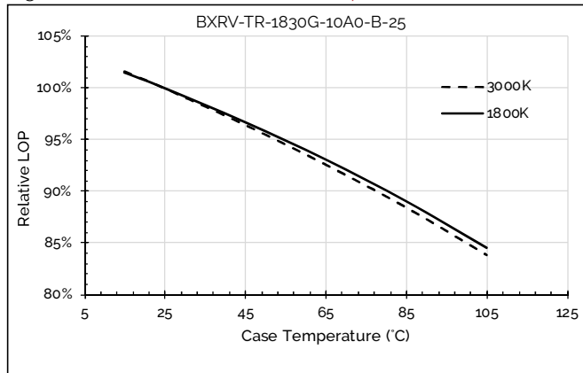
Figure 9: Relative Flux vs. Case Temperature
