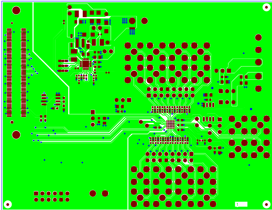
Figure 17. Top PCB Layer
