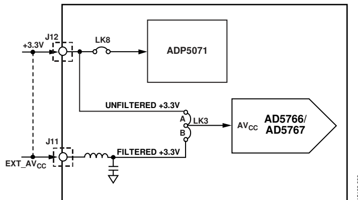
Figure 6. AV_{CC} Selection
