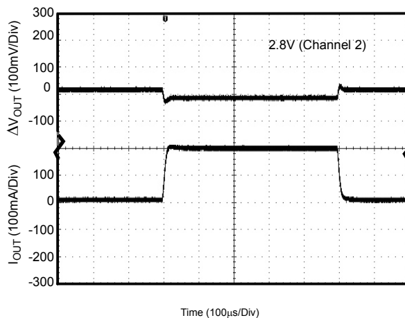
Figure 39. Load Transient
