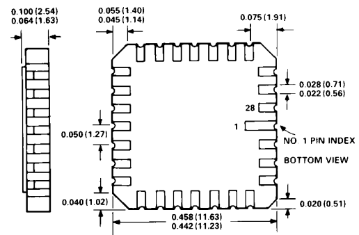
28-Pin LCC
