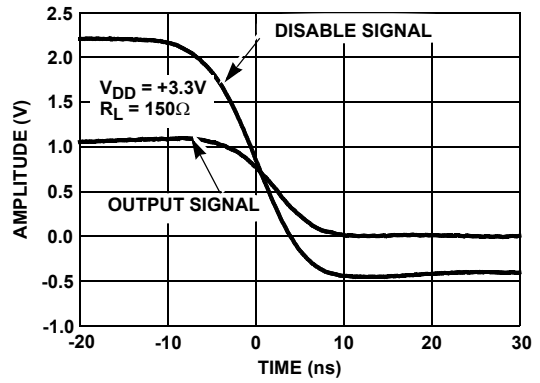
FIGURE 14. DISABLE TIME
