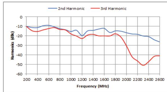
Harmonics (@ Psat)
