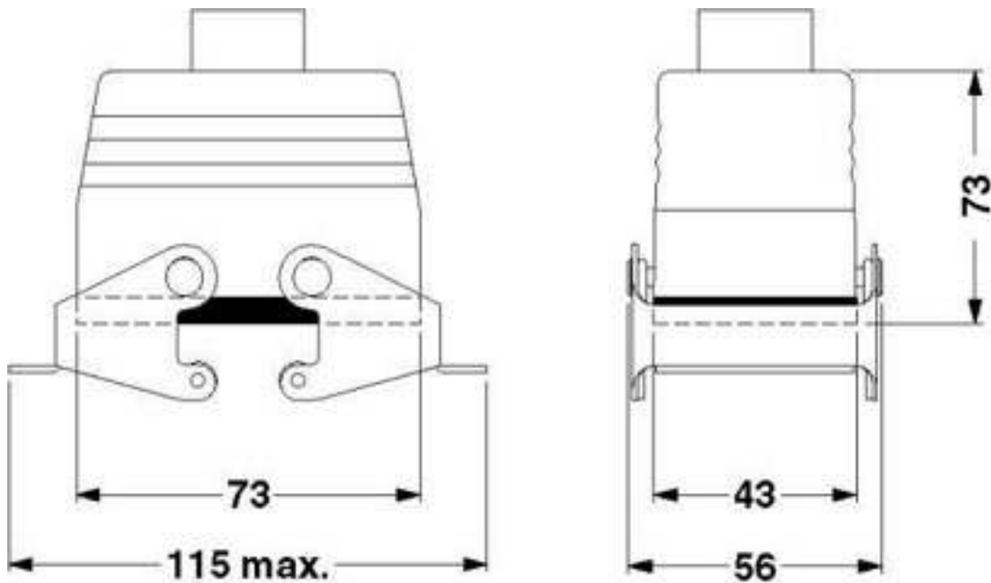
Dimensioned drawing
