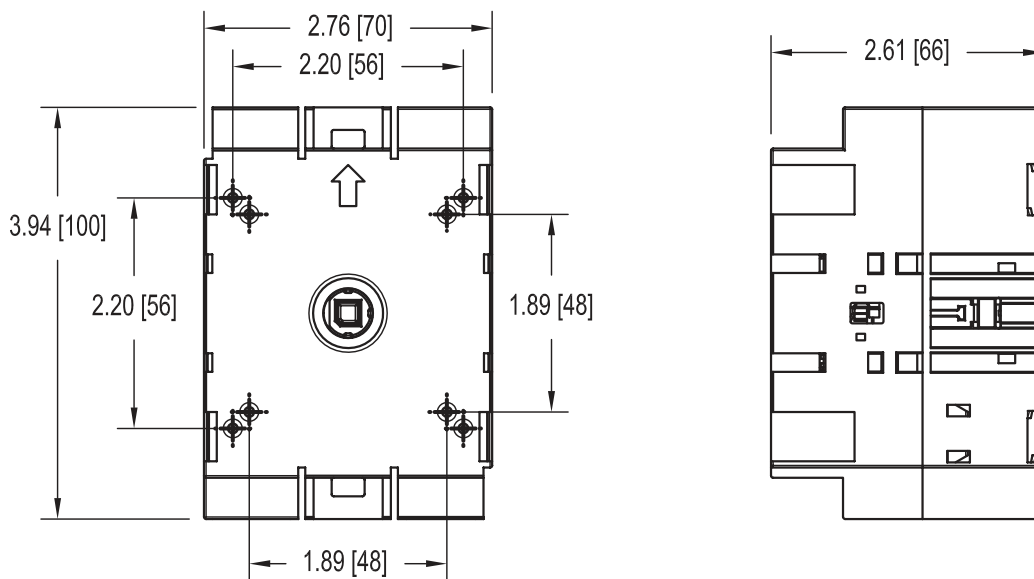
CDNF30A3D, CDFN60A3D, CDFN100A3D — door mounted switch
