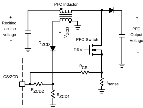
Figure 14. ZCD Winding Implementation
