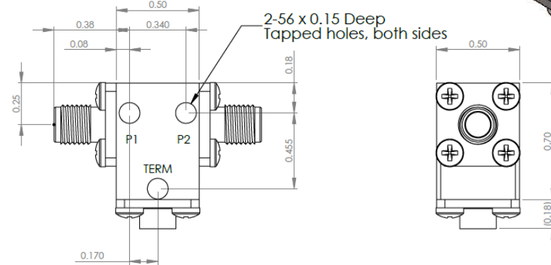
DVI1722-3 Dimensions
