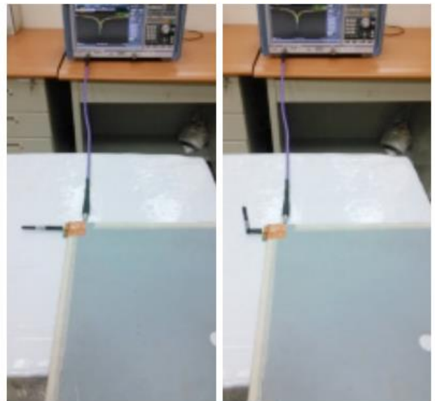
Antenna straight
