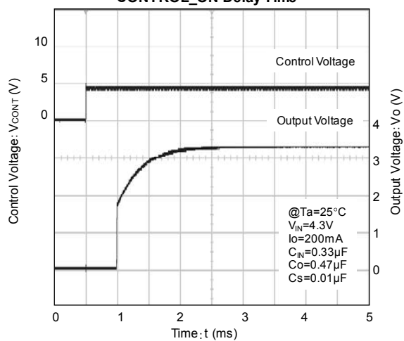
CONTROL_ON Delay Time
