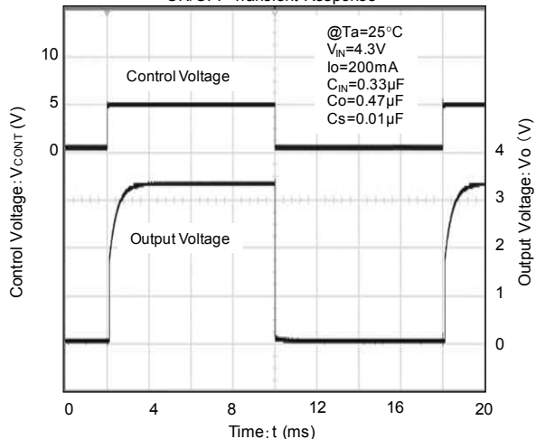
ON/OFF Transient Response
