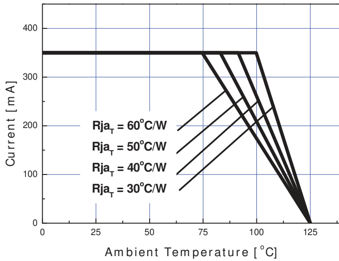
1-4. Photosynthetic Red ( T_{JMAX} = 125\text{ }^{\circ}\text{C} , @700mA)
