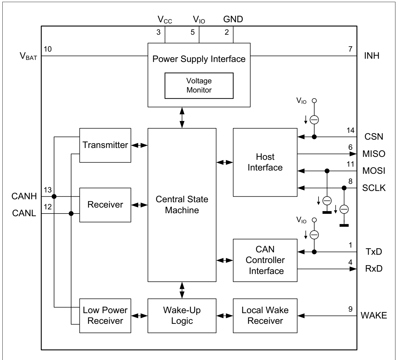
Figure 1 Block Diagram
