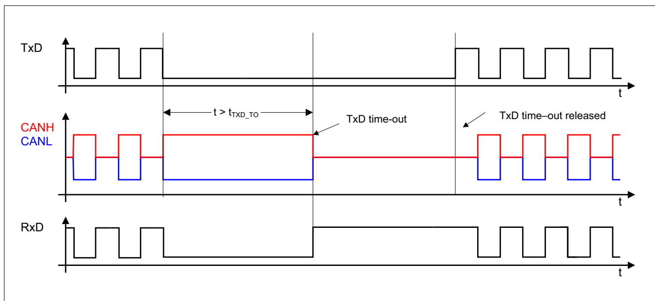
Figure 34 TxD time-out function
