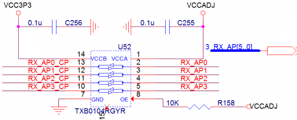
Figure 3-4 Voltage translation of audio data for receiver
