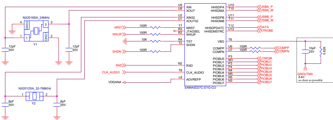
Figure 5-3. SAMA5D27C-D1G-CU System Schematic
