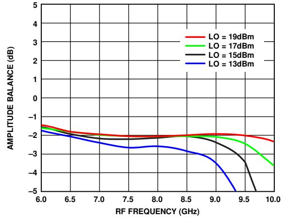
Figure 75. Amplitude Balance vs. RF Frequency at Various LO Powers, T_A = 25^\circ\text{C}
