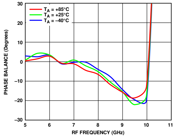
Figure 74. Phase Balance vs. RF Frequency at Various Temperatures
