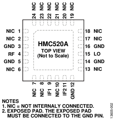
Figure 2. Pin Configuration
