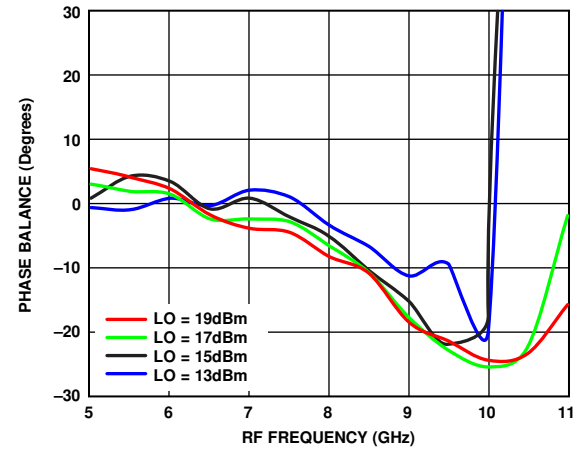
Figure 76. Phase Balance vs. RF Frequency at Various LO Powers, T_A = 25^\circ\text{C}
