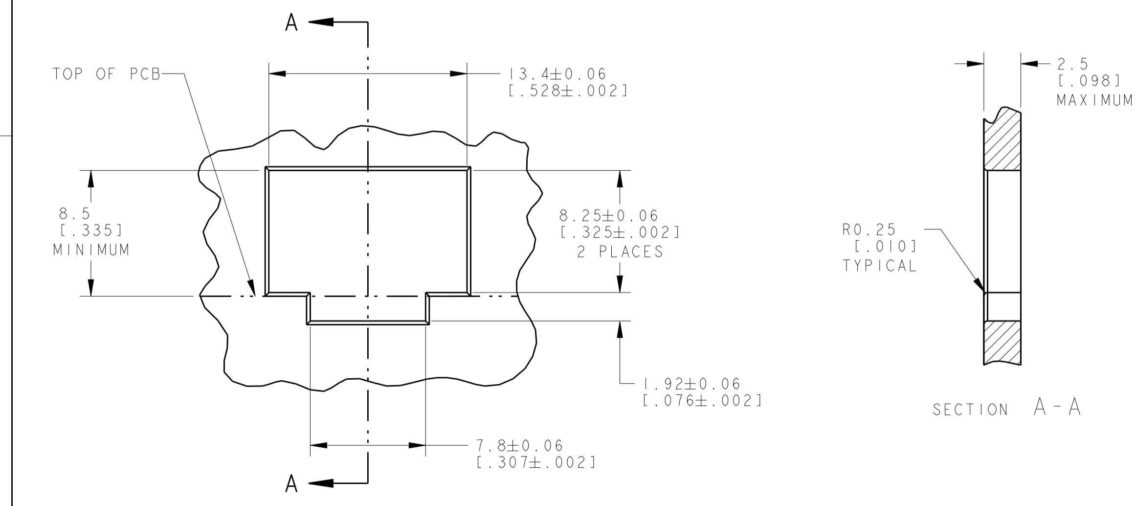
SUGGESTED PANEL CUTOUT SCALE 4:1
