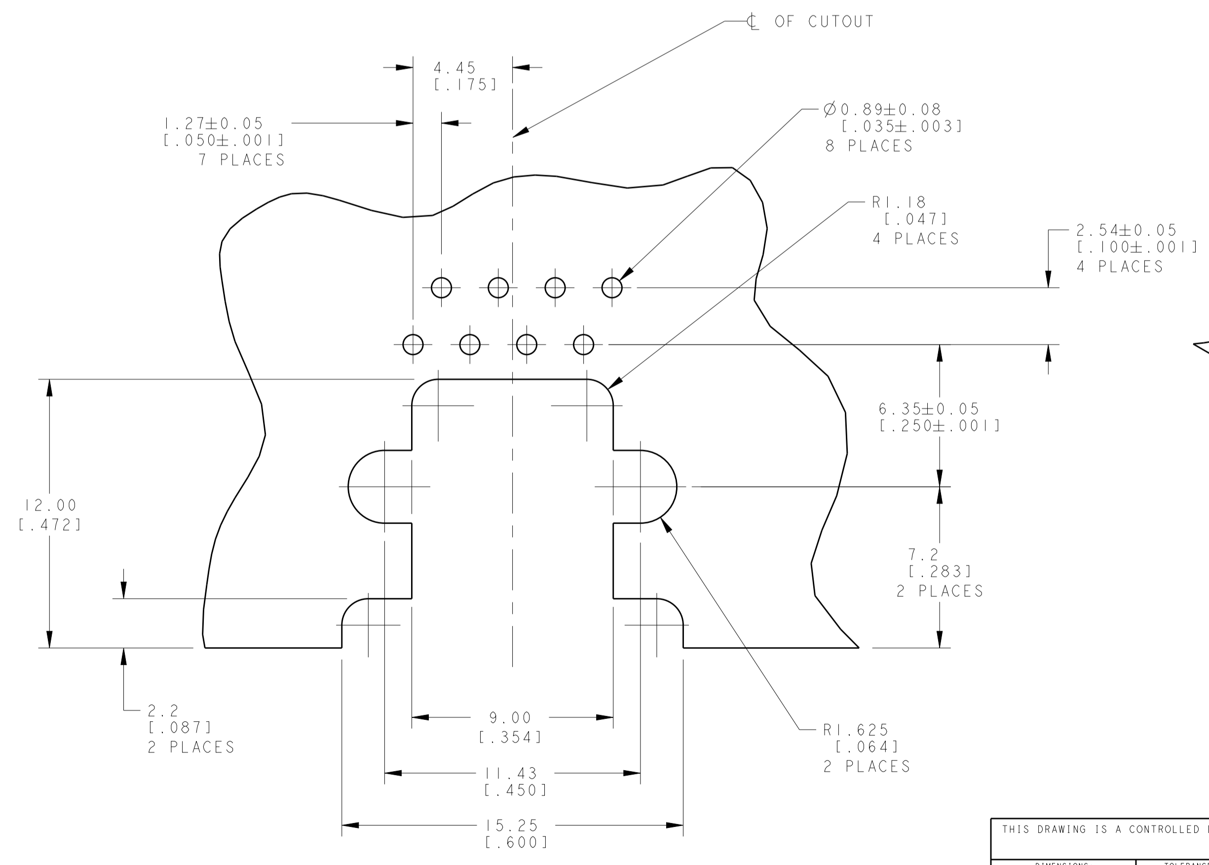
SUGGESTED PRINTED CIRCUIT BOARD LAYOUT COMPONENT SIDE SCALE 6:1
