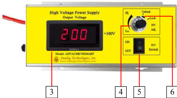
Figure 3. Front Panel
