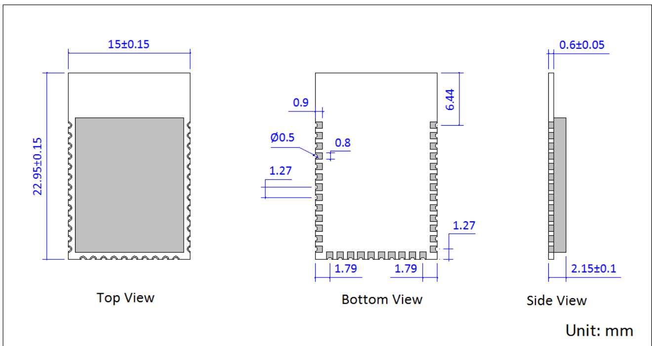
Figure 7-1. Mechanical Drawing
