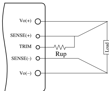
Figure 18. Circuit to Increase Output Voltage
