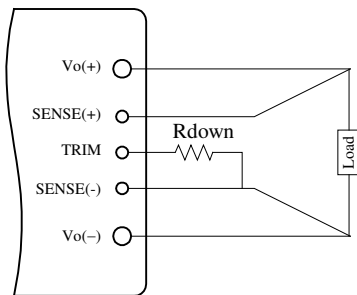
Figure 17. Circuit to Decrease Output Voltage
