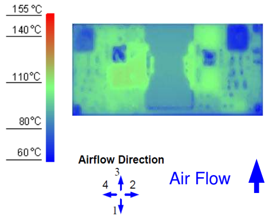
Figure 12. Thermal Image for Airflow Direction 3 (5A output, 55°C ambient, 200 LFM, typical V_{in} , open frame, socket interface)
