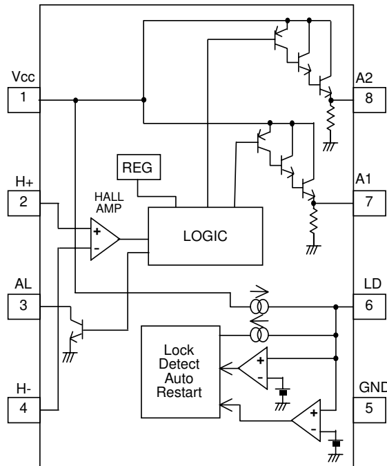
Fig.2 Block diagram
