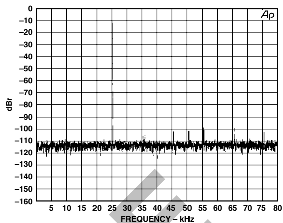
Figure 26. Wideband Plot, 25 kHz Input, 2 Interpolation, SR 192 kHz
