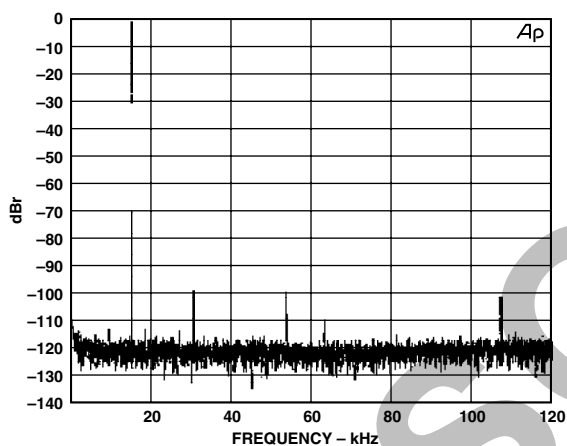
Figure 24. Wideband Plot, 15 kHz Input, 8 Interpolation, SR 48 kHz
