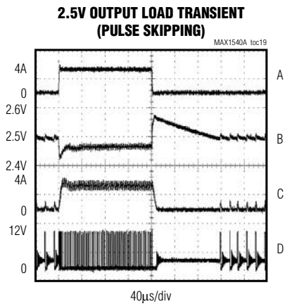
A. I_{OUT2} = 0.1A TO 4A, 5A/div C. INDUCTOR CURRENT, 5A/div B. V_{OUT2} = 2.5V , 100mV/div D. LX2, 10V/div
