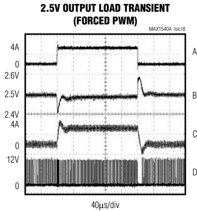
A. I_{OUT2} = 0 TO 4A, 5A/div C. INDUCTOR CURRENT, 5A/div B. V_{OUT2} = 2.5V , 100mV/div D. LX2, 10V/div
