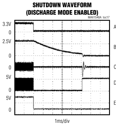
A. ON2, 5V/div D. DL2, 5V/div B. OUT2, 2V/div E. PGOOD2, 5V/div C. INDUCTOR CURRENT, 2A/div
