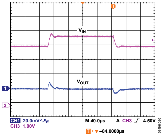
Figure 23. Response to Line Transient, V_{OUT} = 3.3\text{ V} , V_{IN} = 4.0\text{ V} to 4.8\text{ V} , PWM Mode
