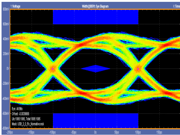
Figure 11. USB3.0 Eye Diagram with and without ESD8504G. 5 Gb/s
